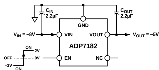
Figure 1. ADP7182 with Fixed Output Voltage, V_{\text{OUT}} = -5\text{ V}
