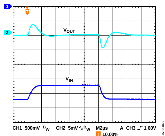
Figure 65. Line Transient Response, 500mV Step, V_{OUT} = -1.8V , I_{LOAD} = -200mA
