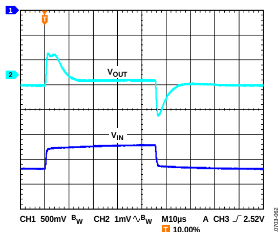
Figure 64. Line Transient Response, 500mV Step, V_{OUT} = -1.22V , I_{LOAD} = -10mA
