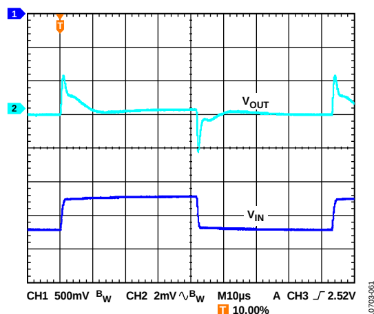
Figure 63. Line Transient Response, 500mV Step, V_{OUT} = -1.22V , I_{LOAD} = -200mA
