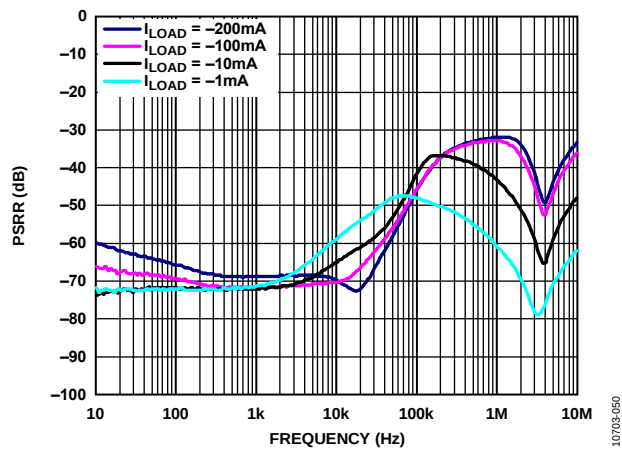
Figure 52. Power Supply Rejection Ratio (PSRR) vs. Frequency, V_{OUT} = -1.8\text{ V} vs. Different Load Currents ( I_{LOAD} ), V_{IN} = -2.8\text{ V}
