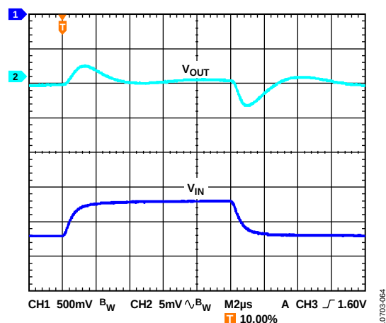
Figure 66. Line Transient Response, 500mV Step, V_{OUT} = -1.8V , I_{LOAD} = -10mA
