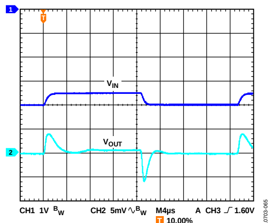
Figure 67. Line Transient Response, 500mV Step, V_{OUT} = -3V , I_{LOAD} = -200mA
