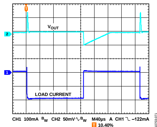
Figure 73. Load Transient Response, V_{OUT} = -1.22 V, I_{LOAD} = -1 mA to -200 mA, Load Step = 1 A/ \mu s
