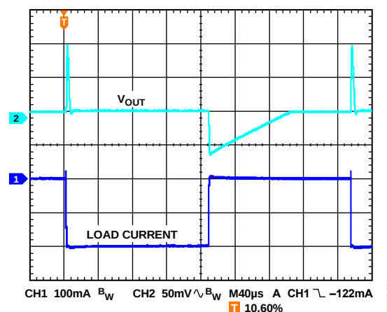
Figure 74. Load Transient Response, V_{OUT} = -3 V, I_{LOAD} = -1 mA to -200 mA, Load Step = 1 A/ \mu s
