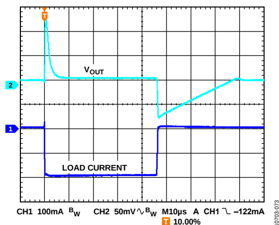
Figure 75. Load Transient Response, V_{OUT} = -5 V, I_{LOAD} = -1 mA to -200 mA, Load Step = 1 A/ \mu s
