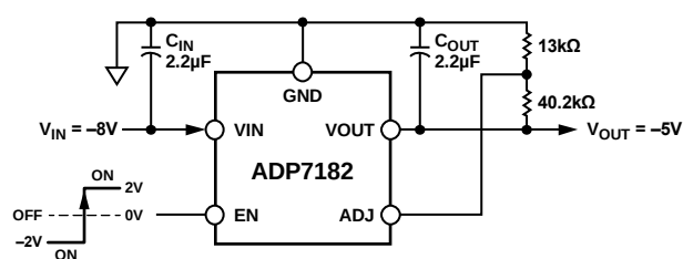
Figure 2. ADP7182 with Adjustable Output Voltage, V_{\text{OUT}} = -5\text{ V}
