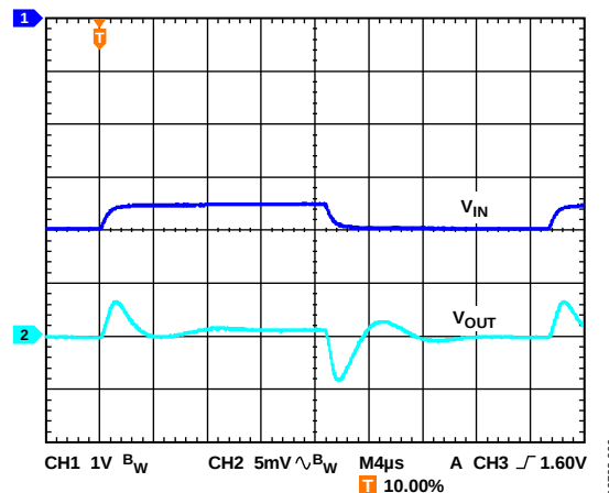
Figure 68. Line Transient Response, 500mV Step, V_{OUT} = -3V , I_{LOAD} = -10mA
