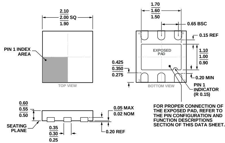
Figure 104. 6-Lead Lead Frame Chip Scale Package [LFCSP] 2.00 mm × 2.00 mm Body and 0.55 Package Height (CP-6-3)
