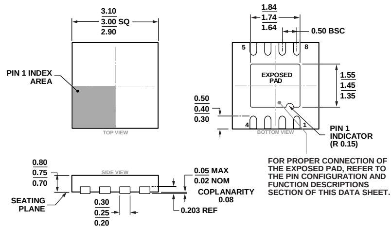
COMPLIANT TO JEDEC STANDARDS MO-229-WEED-4 Figure 105. 8-Lead Lead Frame Chip Scale Package [LFCSP] 3 mm × 3 mm Body and 0.75 Package Height (CP-8-13)
