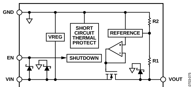
Figure 77. Fixed Output Voltage Internal Block Diagram
