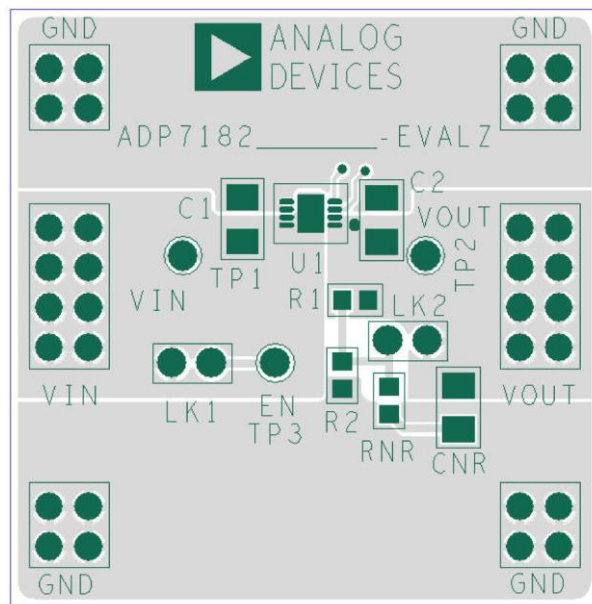
Figure 102. Example of the 8-Lead LFCSP PCB Layout
